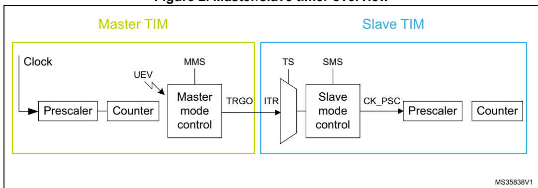
Figure 2. Master/slave timer overview
