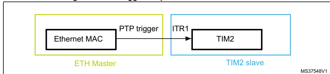
Figure 7. PTP trigger output to TIM2 ITR1 connection
