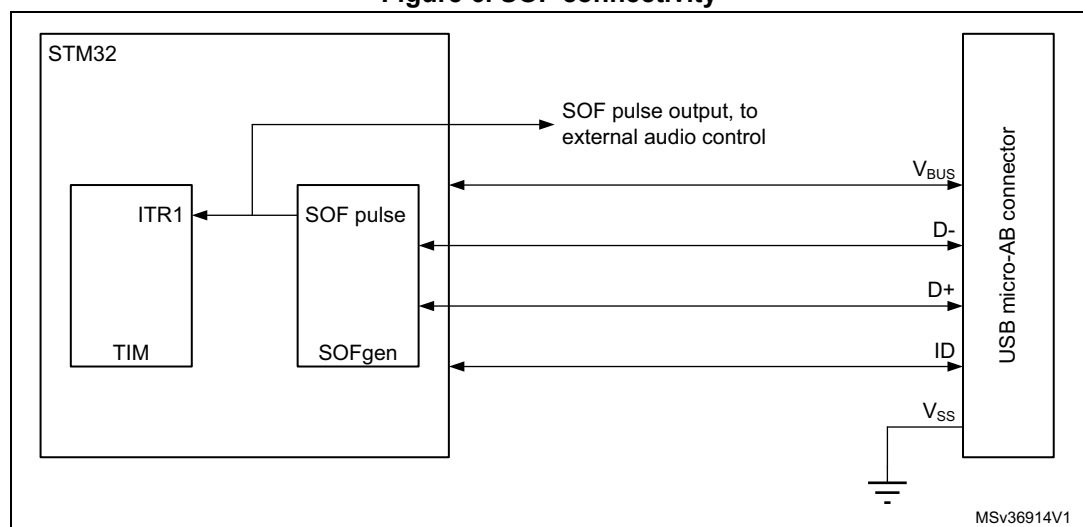
Figure 6. SOF connectivity
