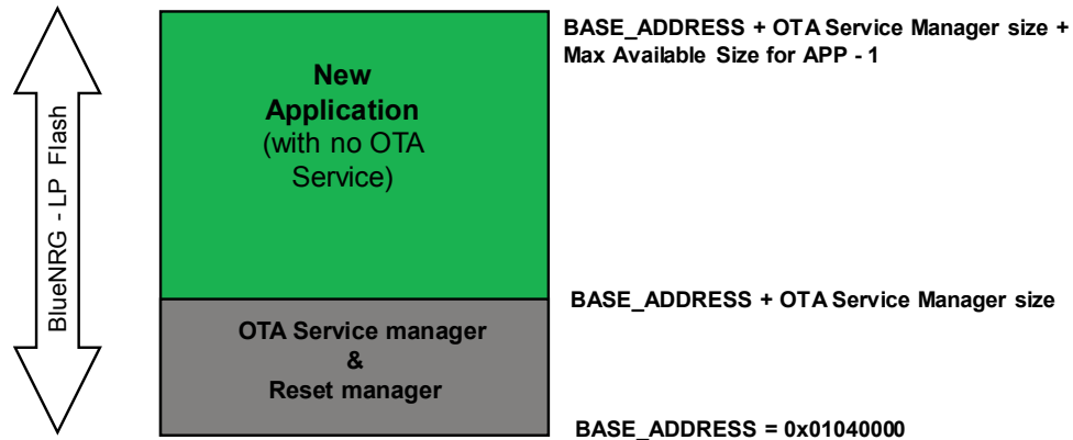
Figure 5. OTA service manager Flash memory layout
