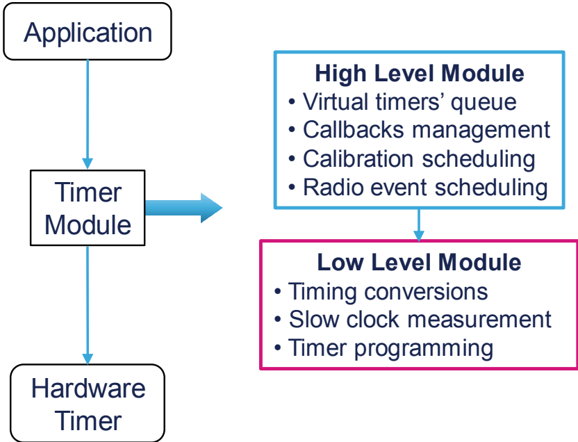
Figure 1. Timer module components
