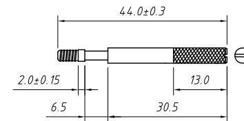
Long screw
