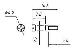
Short screw
