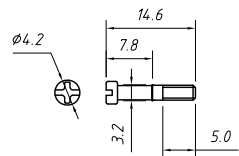
Short screw
